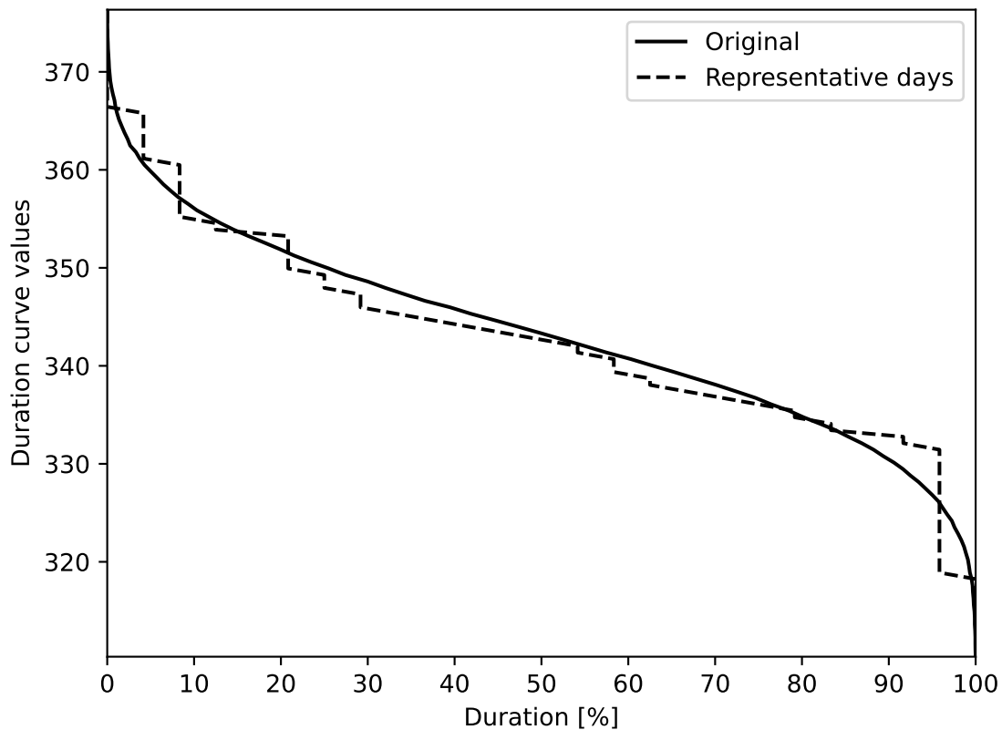
total load
